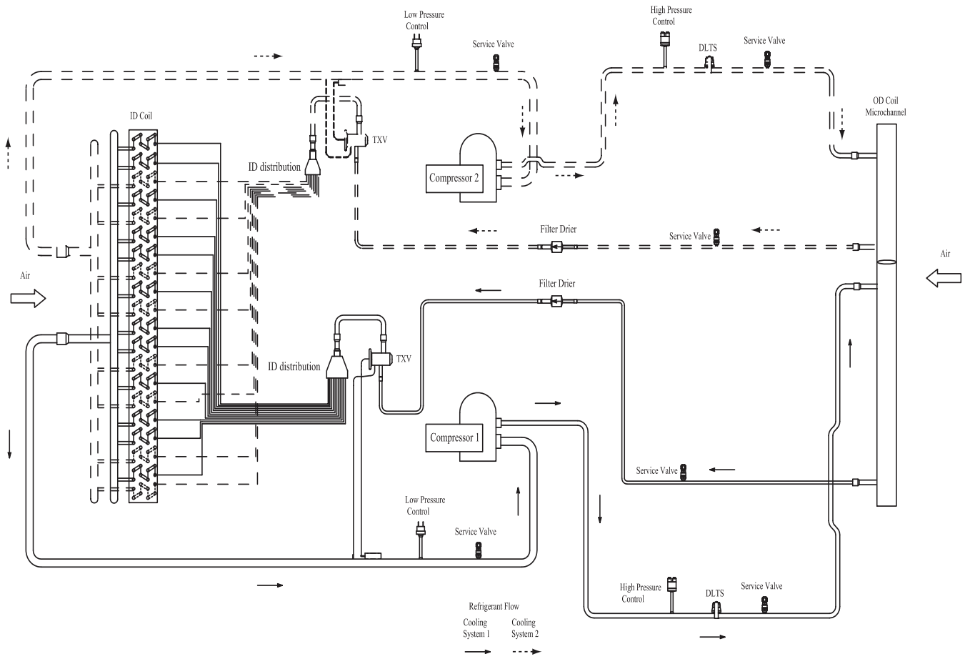
Figure 4. T/YSC120F
